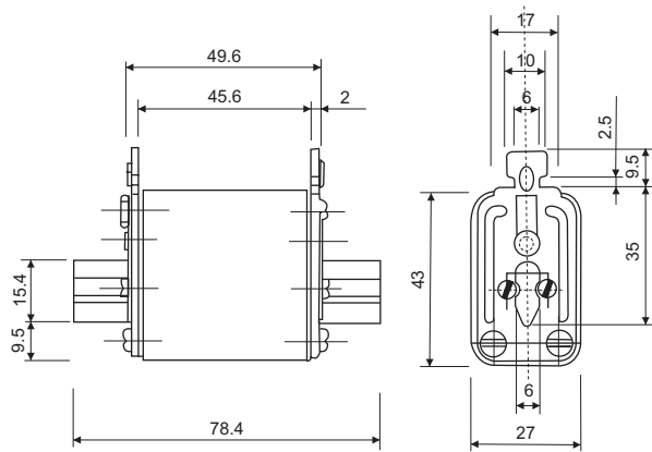
Size 00
