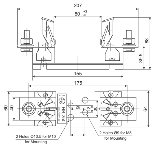
HB 250
